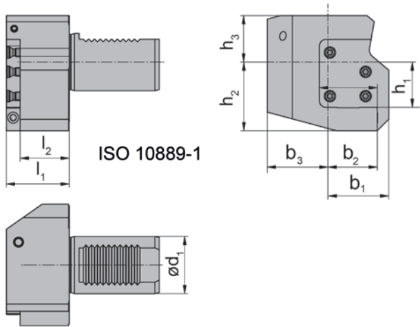
Illustration = Base de support type B1 Figura = Supporto base tipo B1
