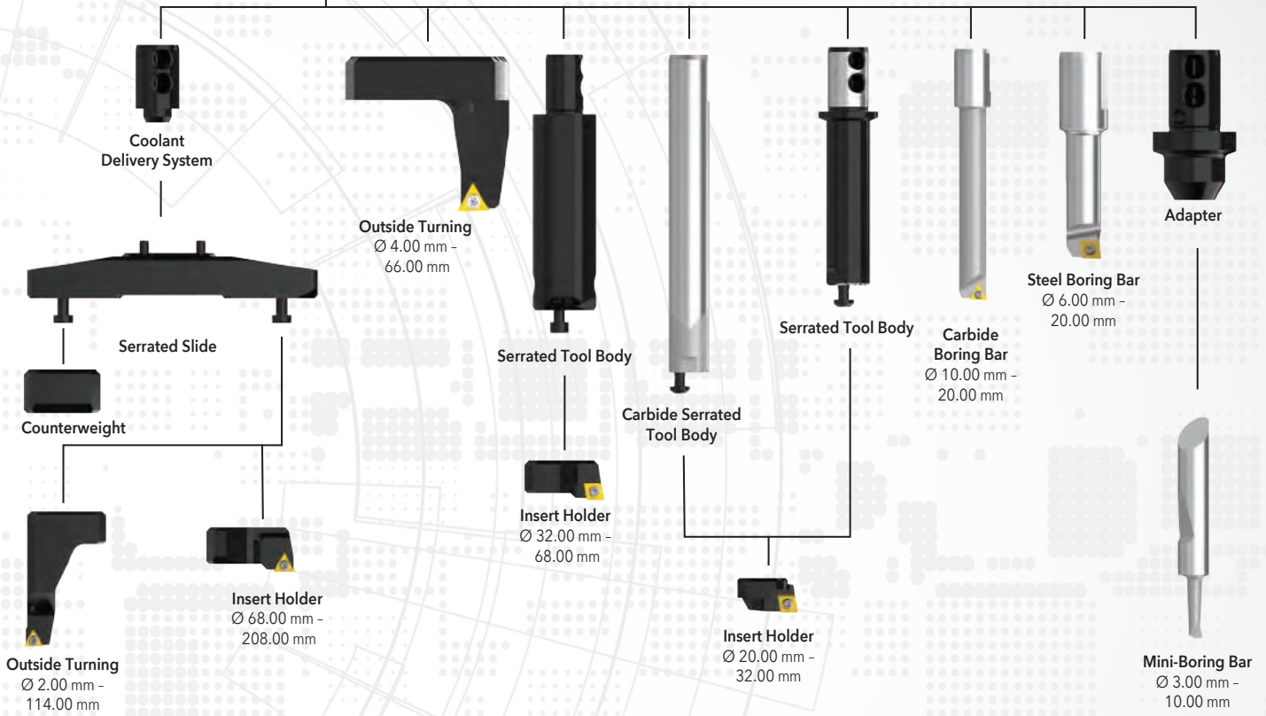
DigiBore Head
